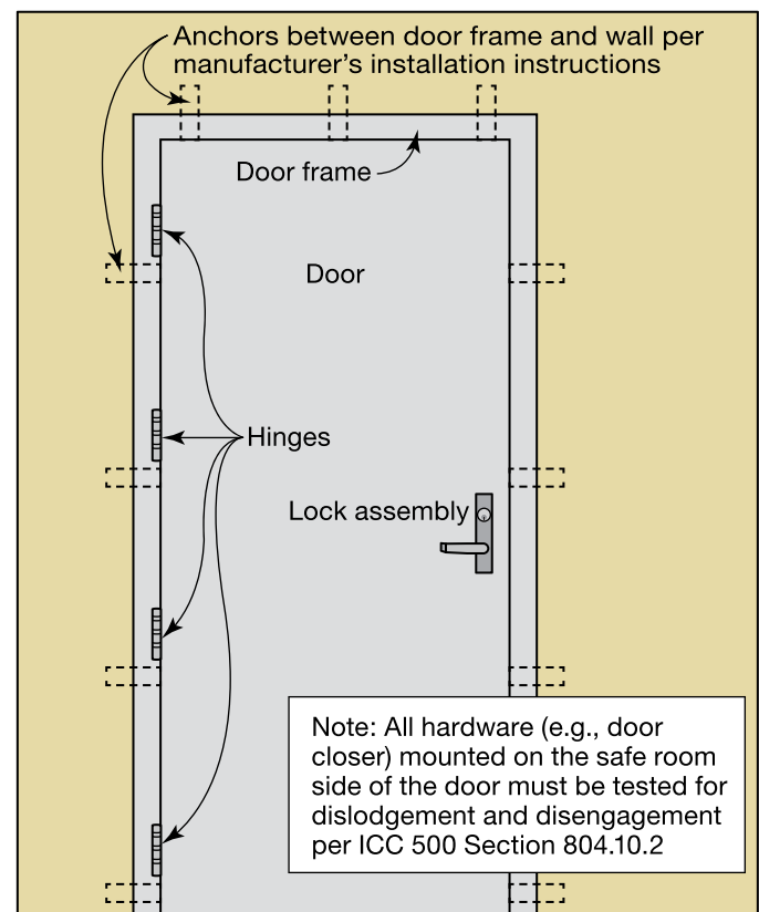
Figure 1: Components of a safe room door assembly
